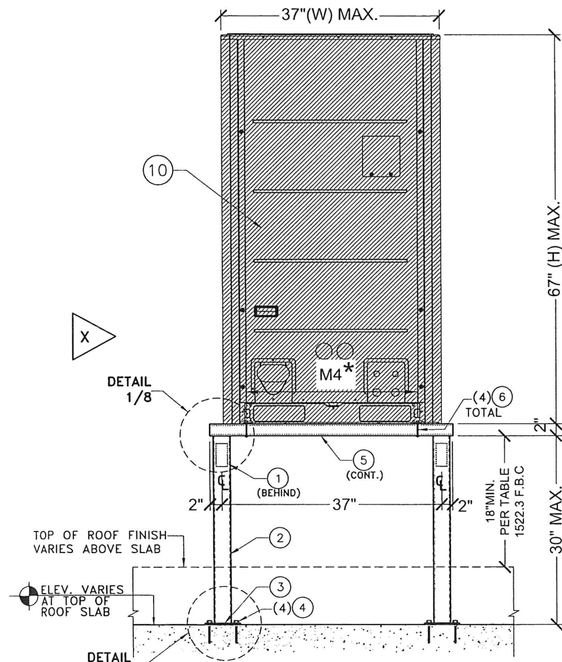
TYP. ELEVATION VRF/VRV-1
