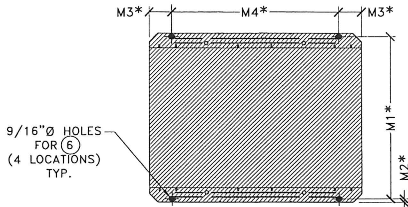
BOTTOM MOUNTING HOLES
