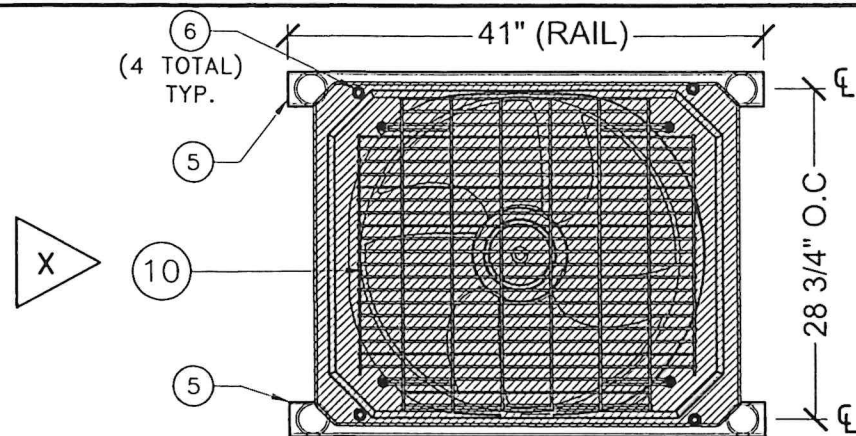
TYP. PLAN VIEW VRF STAND
