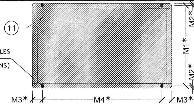
BOTTOM MOUNTING HOLES
